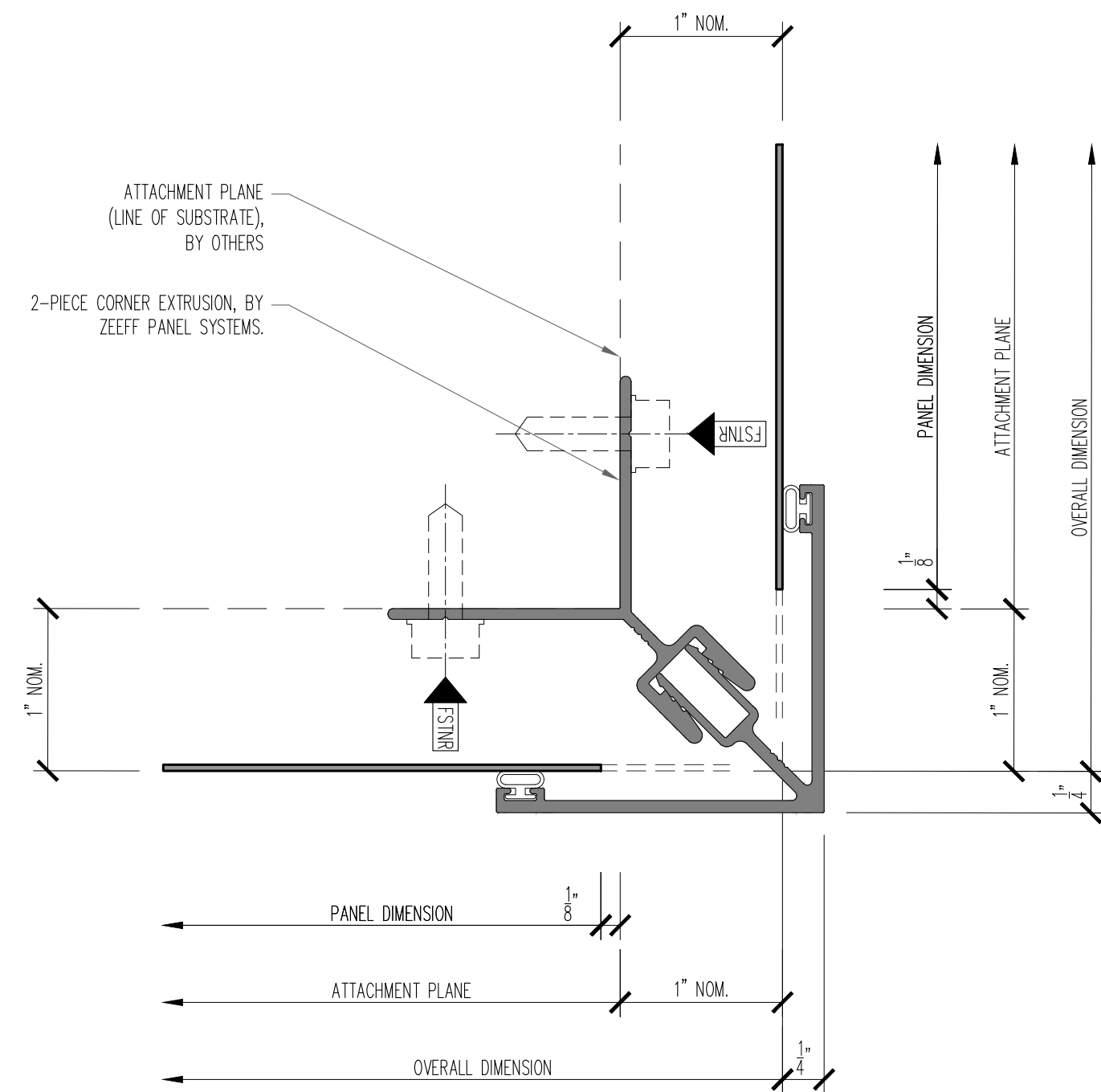
X OUTSIDE CORNER DETAIL SCALE: FULL
