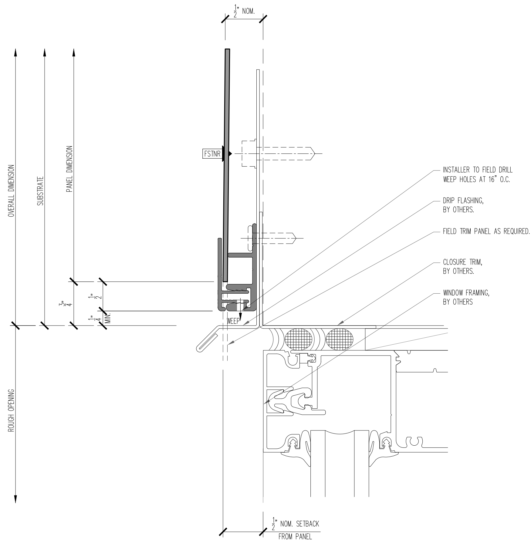
X PANEL BASE DETAIL AT WINDOW / DOOR HEAD SCALE: FULL
